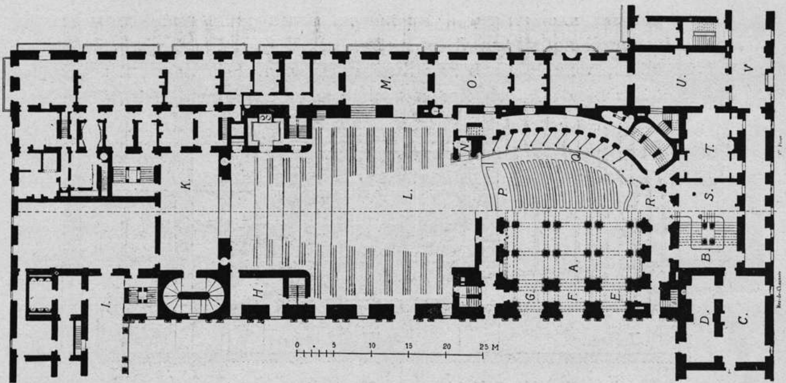
Fig. 64. Das Theater in Turin.
