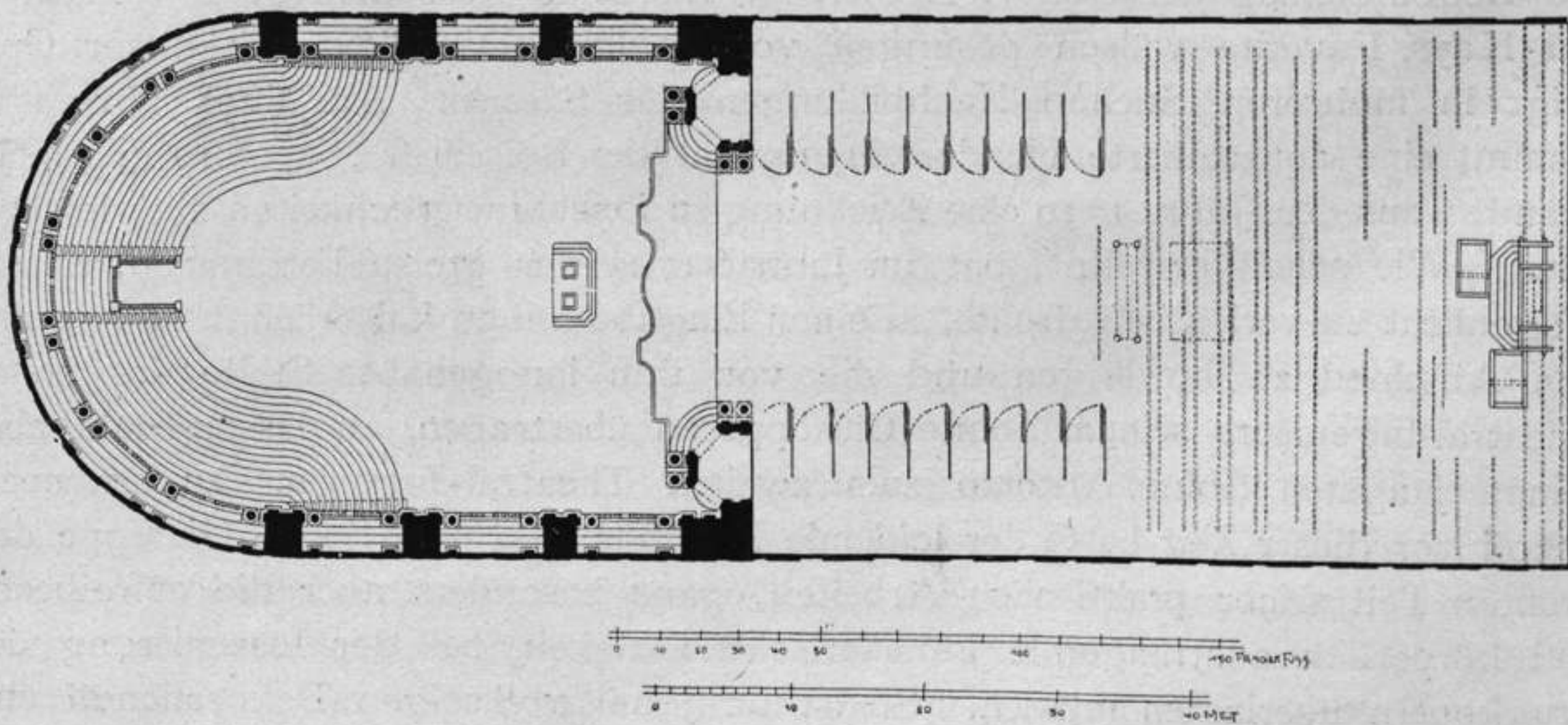
Fig. 105. Offenes Theater in Prag.
